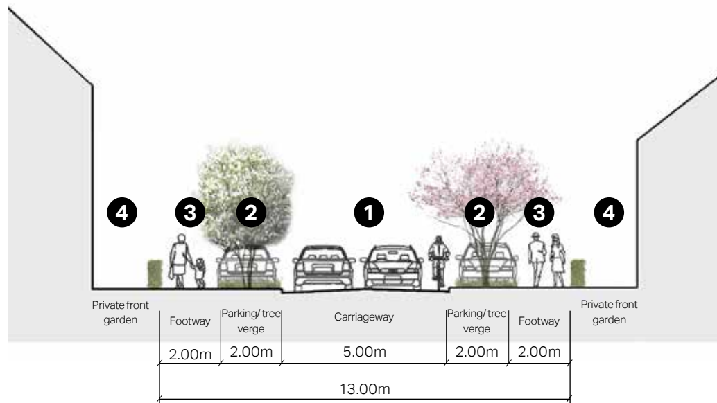
Figure 115: Section showing indicative dimensions for tertiary route. In some places tree verges may be omitted from one or both sides
