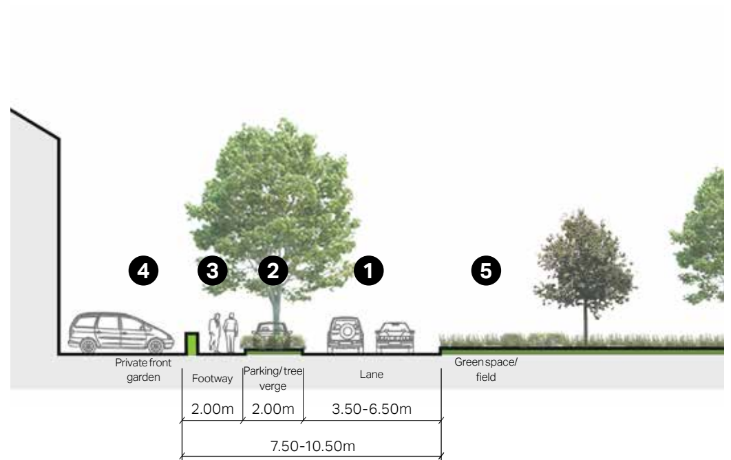
Figure 114: Section showing indicative dimensions for edge lanes. The lane width may vary to discourage speeding or provide space for parking
