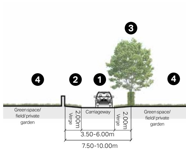
Figure 113: Section showing indicative dimensions for secondary rural route. The carriageway width may vary. This type is found in settlements and rural areas
